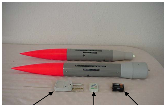
RS92 Digital Radiosonde Datalogger Battery Pack
